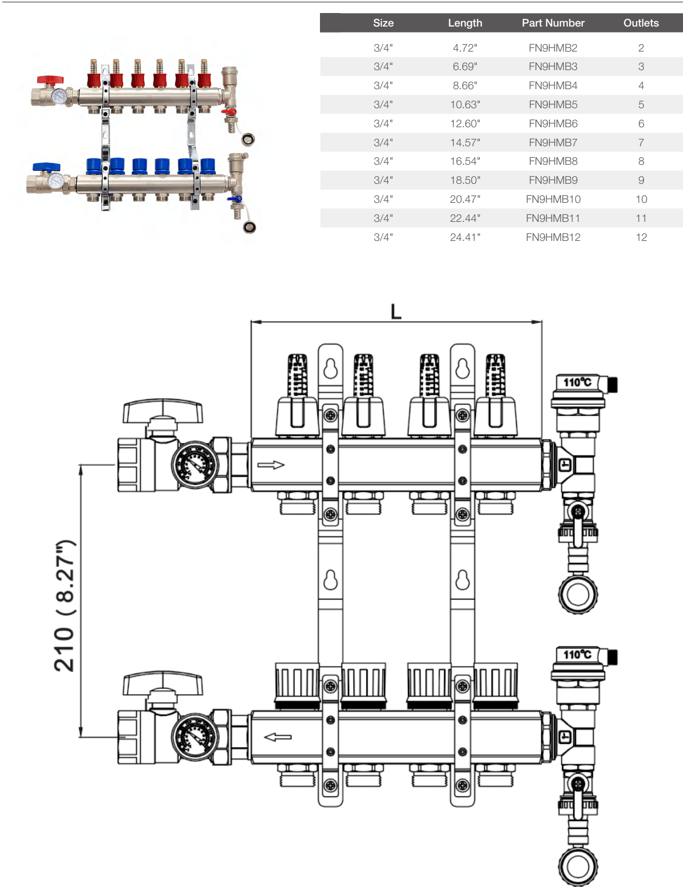
RIIFO FN9 Manifold
