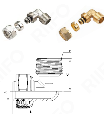
Male elbow
