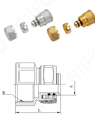
Female straight coupling
