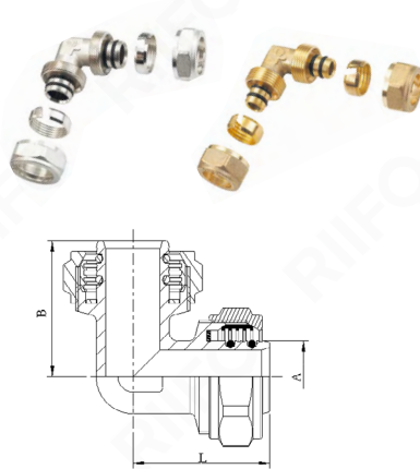
Elbow
