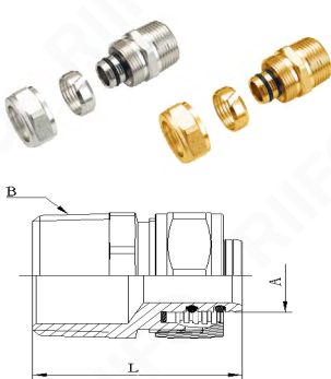
Male straight coupling
