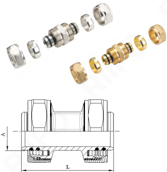
Straight coupling
