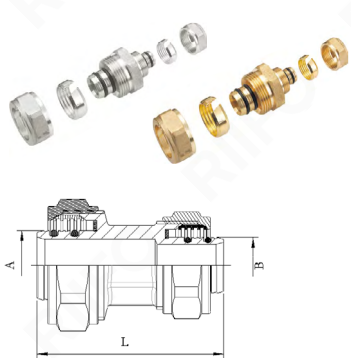
Reducing coupling
