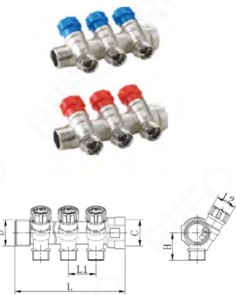
Brass manifolds with stop valves-FS4
