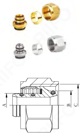
F5 Connector core
